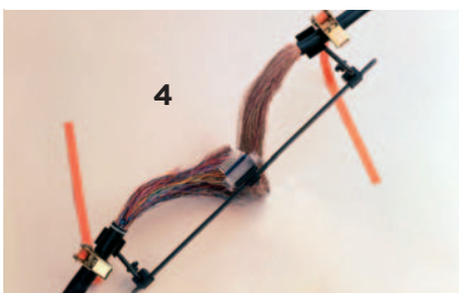
Splicing head with tip-up Column: piece out fixture 1-525421-4
